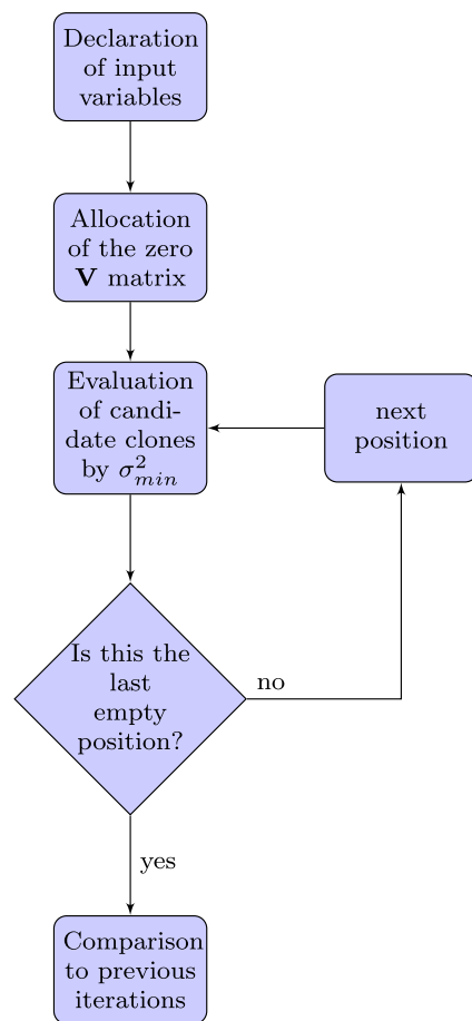
Fig. 6 Schematic description of the ONA's algorithm
